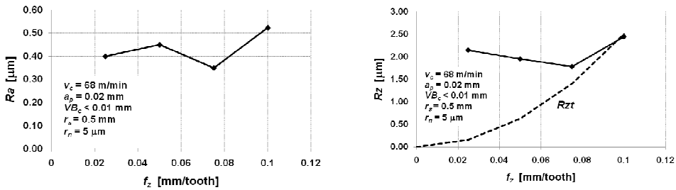
Fig. 16. Surface roughness Ra and Rz in function of feed per tooth f_z
