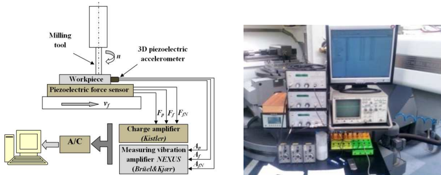
Fig. 5. Block scheme and a view of the cutting force and acceleration of vibrations experimental apparatus
