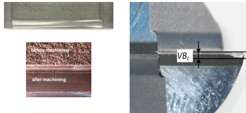
Fig. 4. Tool wear measurement
